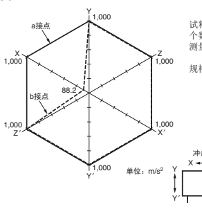
误动作冲击 G6RN-1
